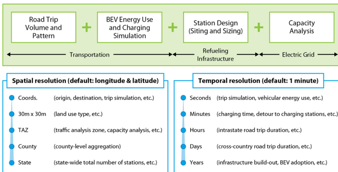
Figure 3. EVI-RoadTrip block diagram for traffic generation, charging behavior simulations, and network design
